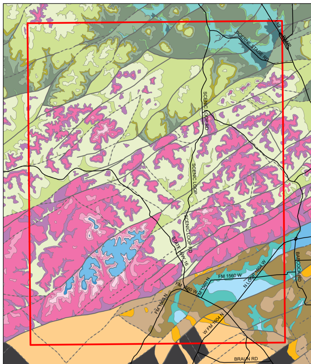
Figure 2-4 Outcrop geology and faults in the study area (modified from Clark et al., 2016).
